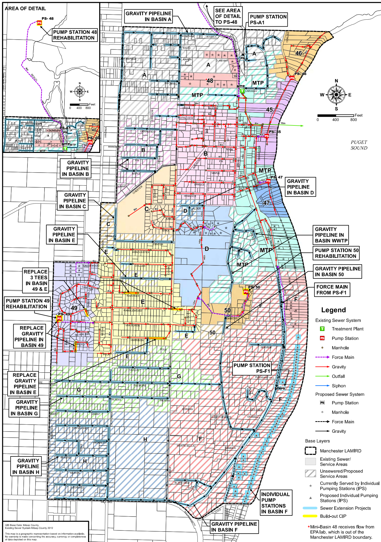
BUILD-OUT CAPITAL IMPROVEMENT PROJECTS MANCHESTER SEWER FACILITIES STRATEGY PLAN Kitsap County October 2014
