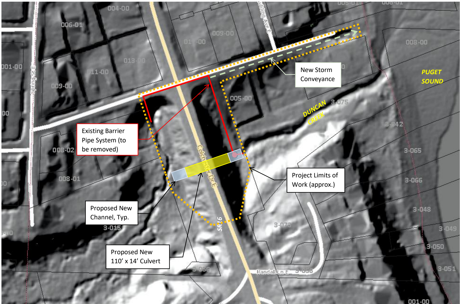
Figure A4. Existing Barrier and Schematic Plan Duncan Creek at Colchester Drive Kitsap County Public Works
