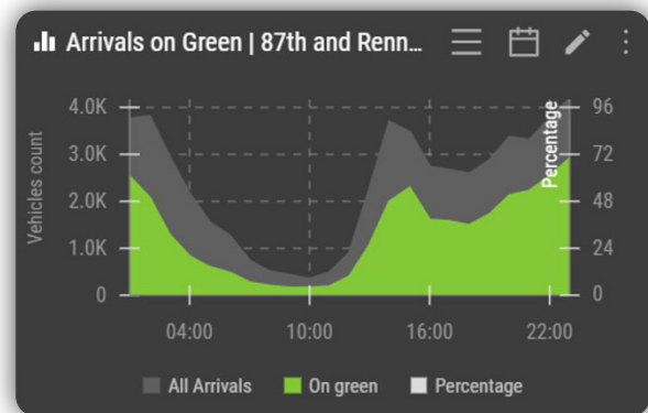
Arrivals on Green Chart
