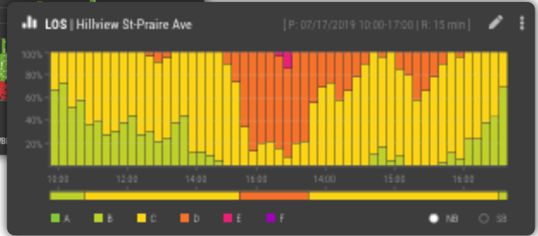
Level of Service Chart
