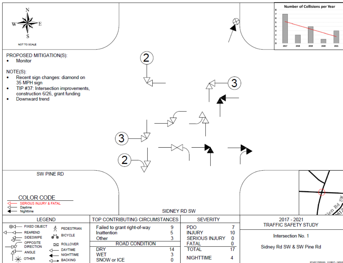
Figure 2.10 – Collision Diagram Example
